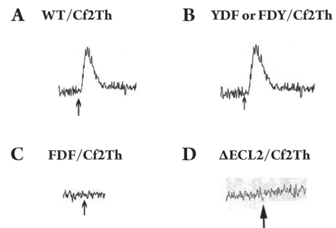
Figure 3. The CXCR3 variant FDF does not mobilize calcium in response to IP-10. Cf2Th cells were transfected with wild-type CXCR3 or with the CXCR3 variants YDF, FDF, or ΔECL2, as described in Materials and Methods. Cells were loaded with the calcium indicator dye Fura-2 and assessed for their ability to mobilize calcium in response to IP-10, which was added at the time points indicated by the arrows. Calcium flux was displayed as the fluorescence ratio of 340 nm to 380 nm. Receptor expression was determined by staining with the anti-FLAG-tag antibody. Mean fluorescence levels were 59.3 for wild-type CXCR3, 48.0 for YDF, 58.9 for FDF and 56.2 for ΔECL2; for mock-transfected cells, the value was 7.7. The data shown are representative of three independent experiments.
